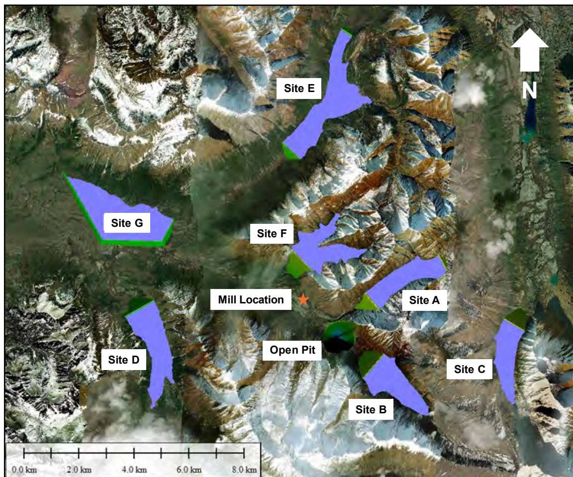
Figure 18-4: Overview of Preliminary Tailings Siting Study Locations
