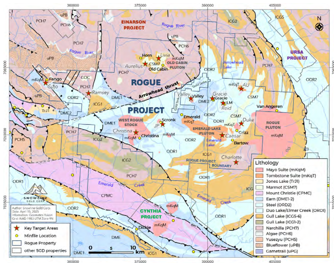
Figure 7-6: Property Geology
