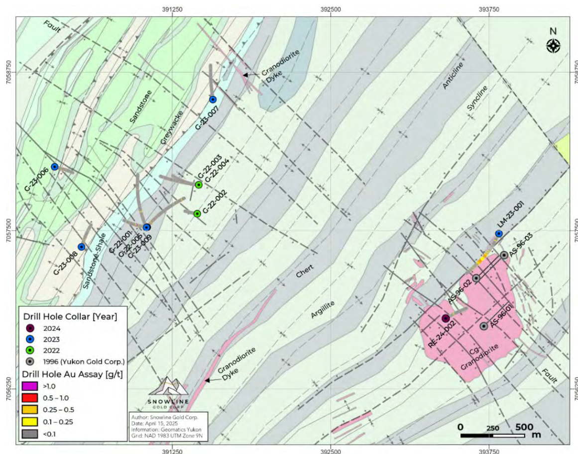
Figure 10-4: Gracie-Reid Drill Assay Over Geology
