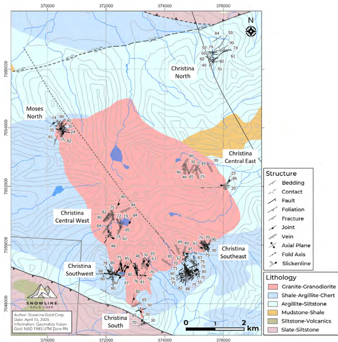
Figure 7-17: Christina Geology
