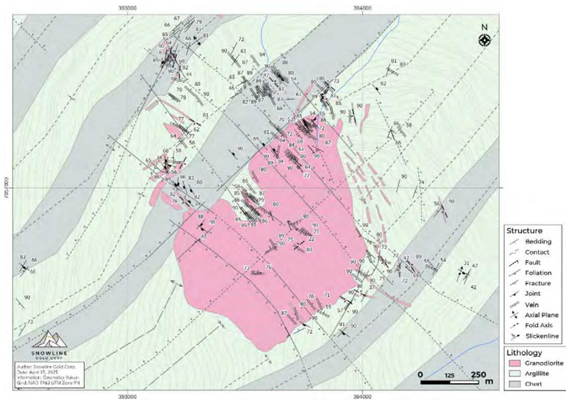
Figure 7-10: Reid Geology
