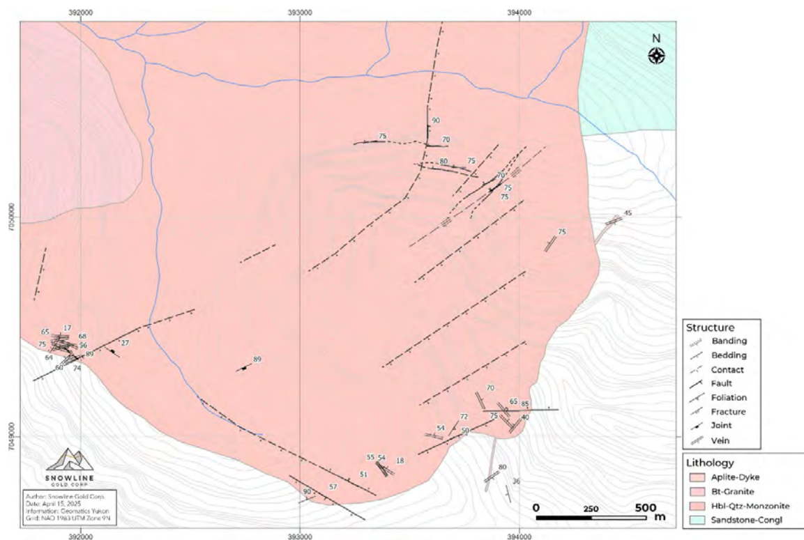
Figure 7-20: Caesar Geology
