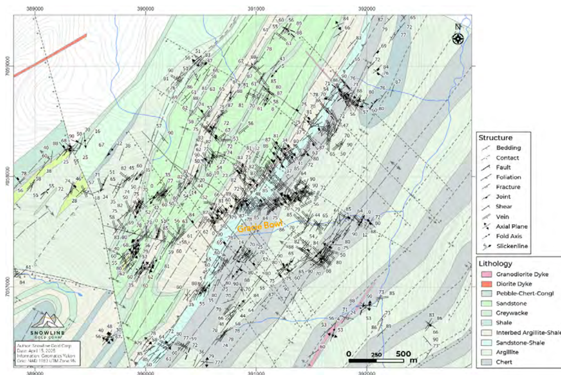
Figure 7-9: Gracie Geology
