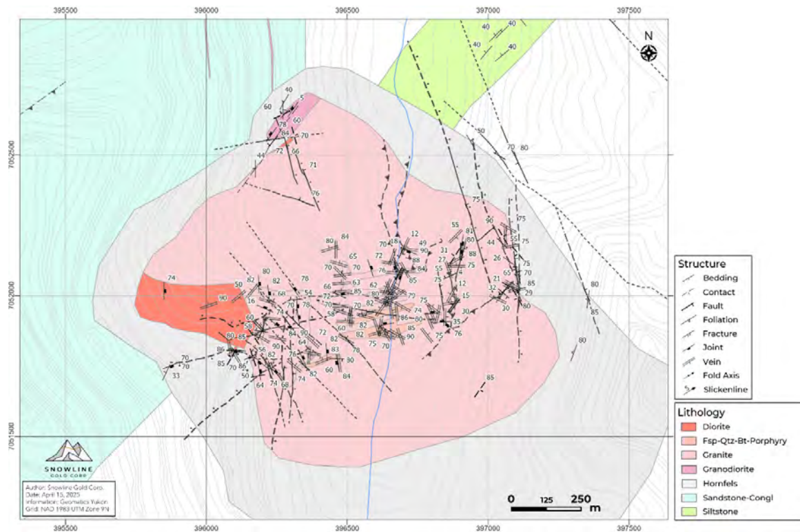
Figure 7-22: Duke Geology
