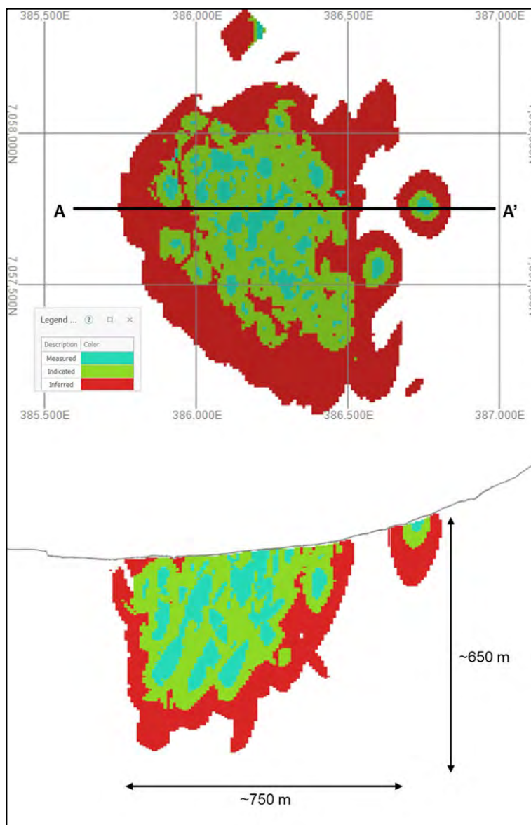
Figure 16-3: Resource Classification
