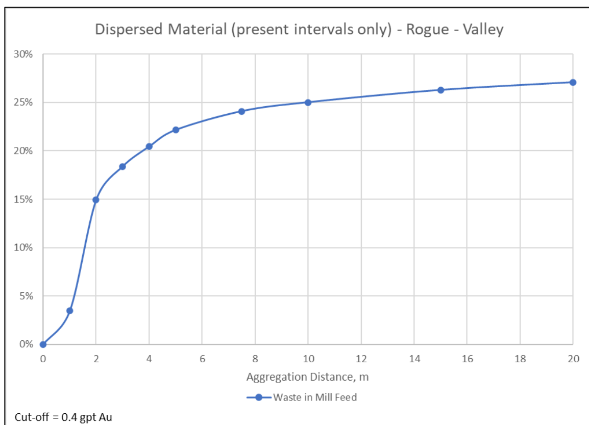
Figure 16-7: Heterogeneity Results
