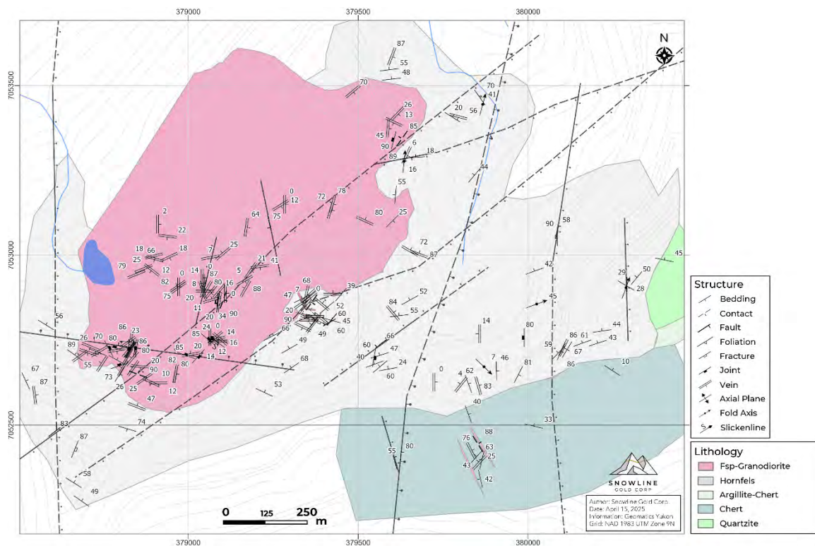
Figure 7-16: JP Geology
