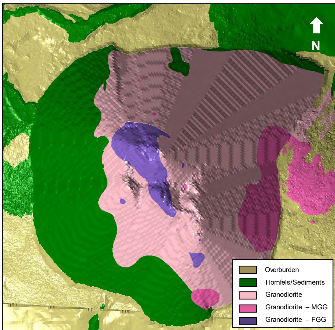
Figure 16-1: Geological Setting of Planned Open Pit Area
