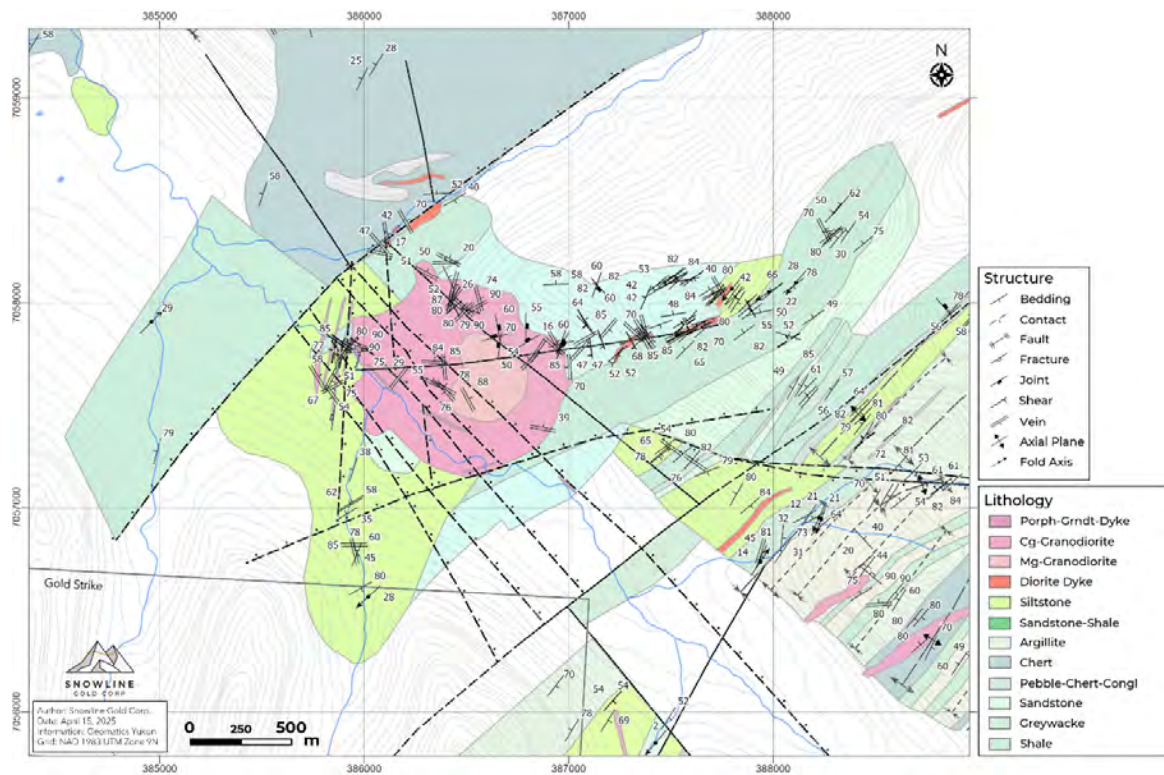
Figure 7-7: Valley Geology
